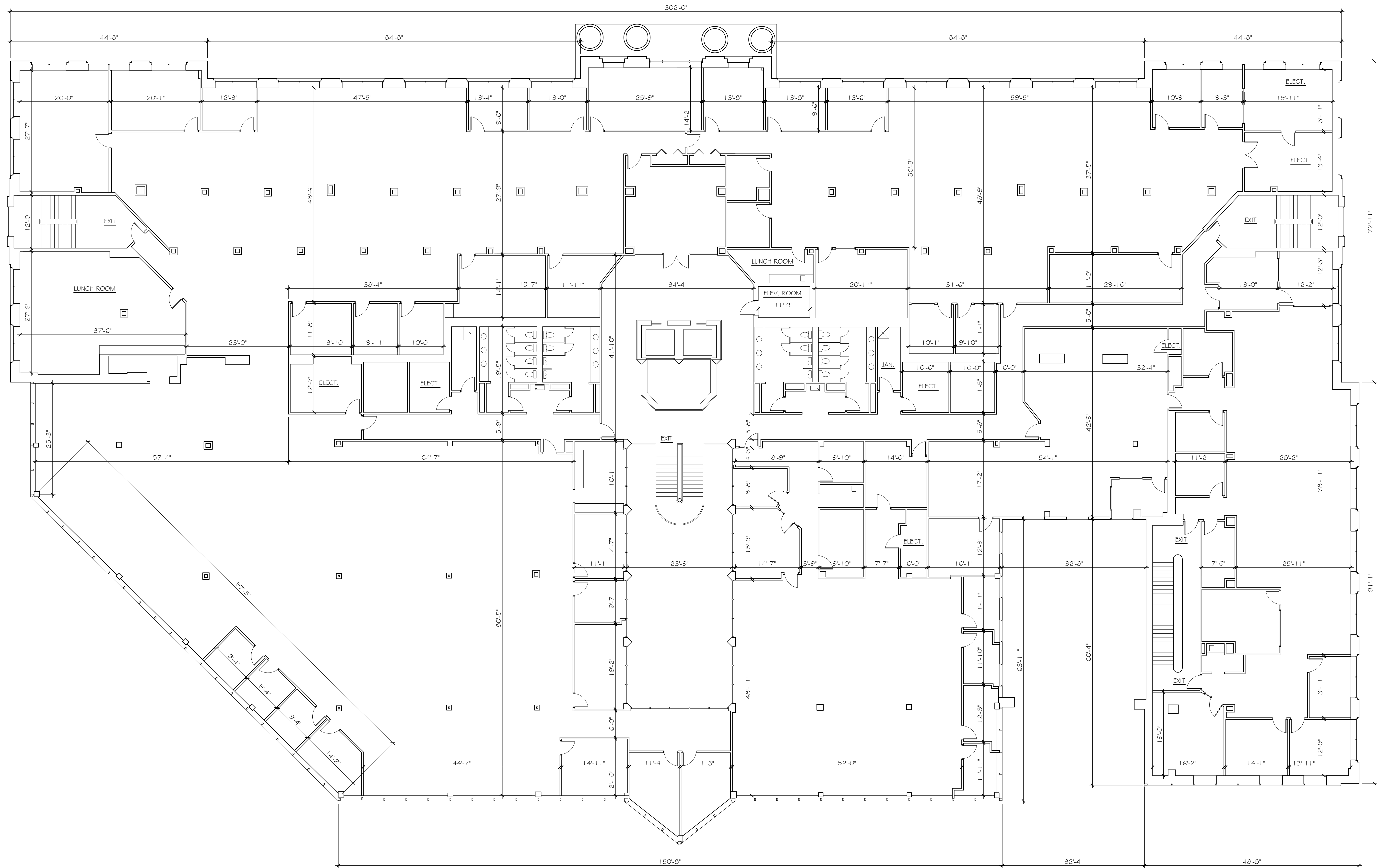
SECOND FLOOR PLAN SCALE: 3/32" = 1'-0"
